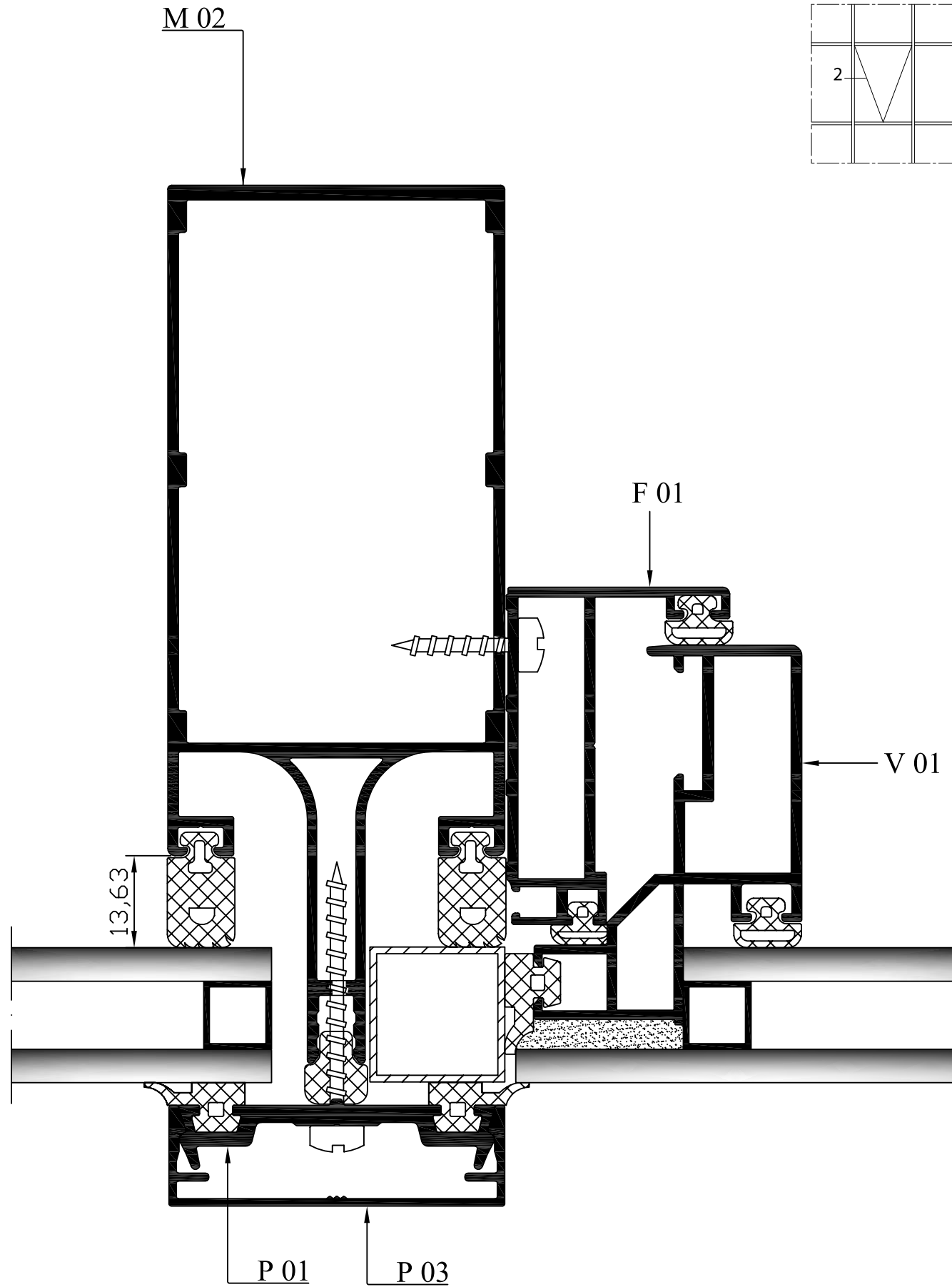
② DETAIL
